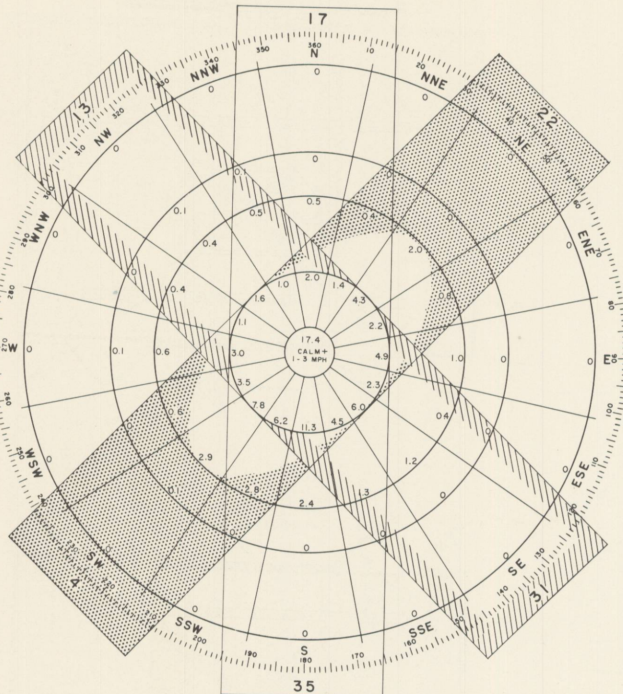
USAF RUNWAY WIND COMPUTER
